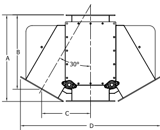
30° Side view
