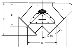
45° Side view
